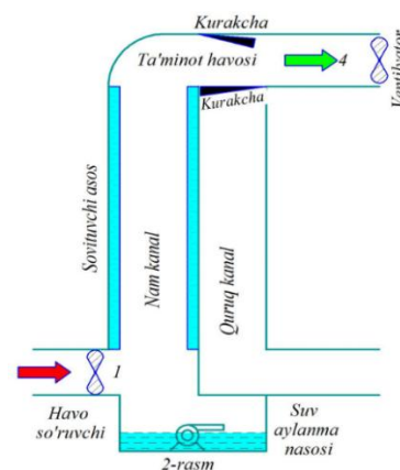
2-rasm. Bevosita bug'lanma sovitgich Fig. 2. Direct evaporative refrigerator
