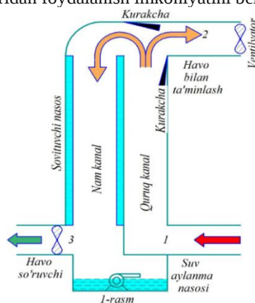
1-rasm. Bilvosita regenerativ bug'lanma sovitgich Fig. 1. Indirect regenerative evaporative refrigerator
